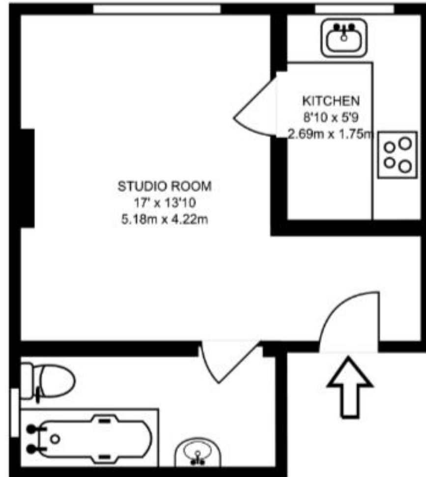
FIRST FLOOR 295 SQ FT/27.38 SQ M
